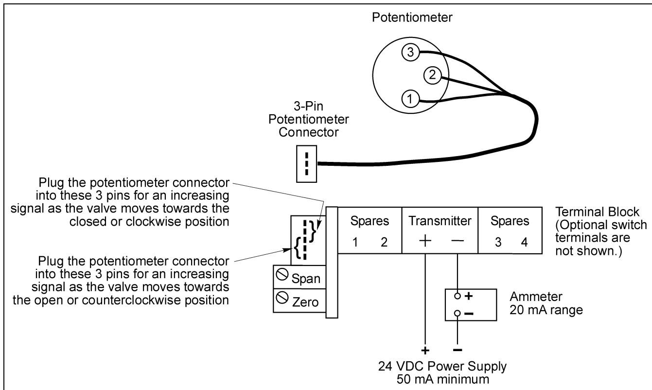
Figure 3—Position Transmitter
