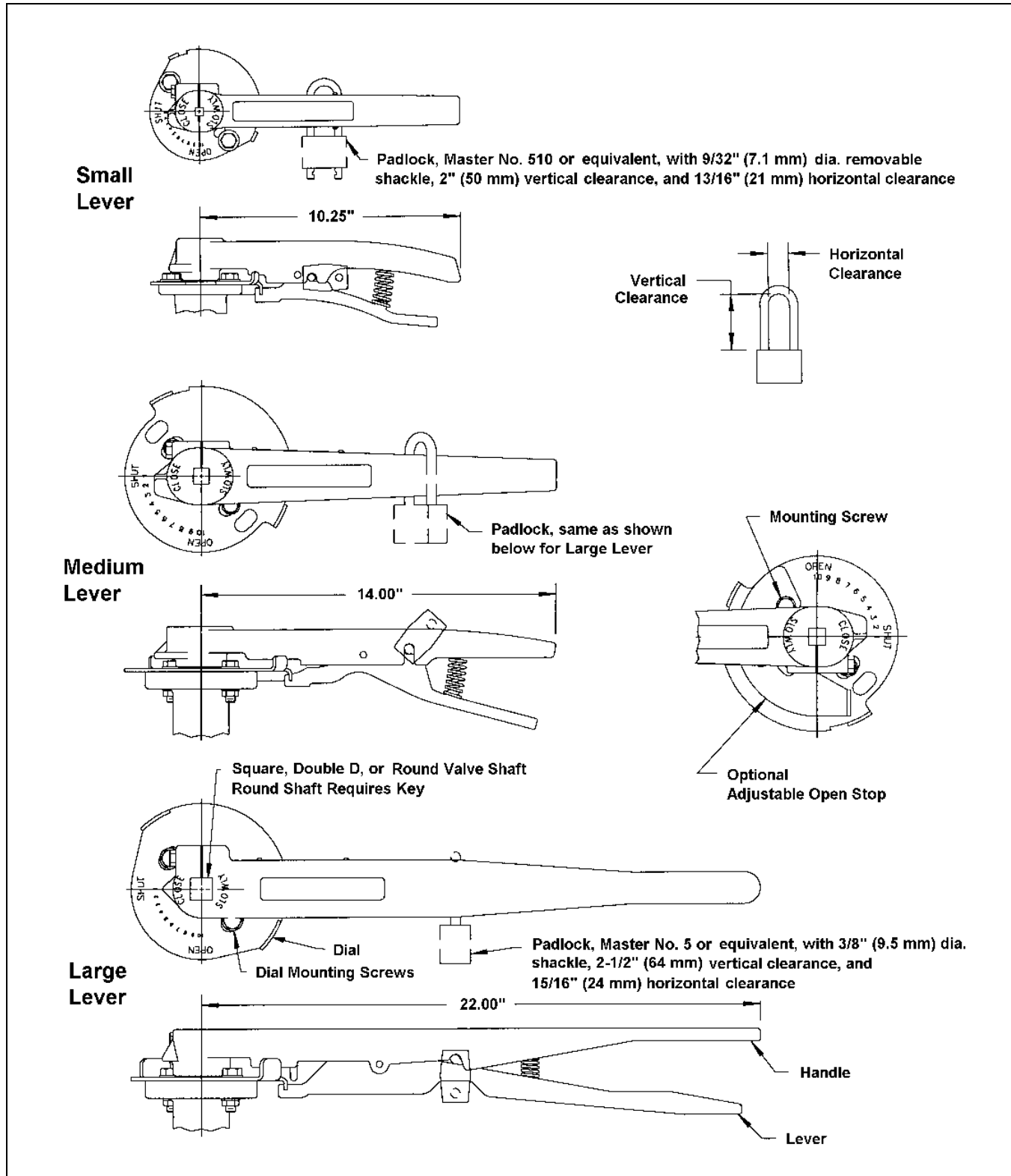
Figure 1 – Actuator Components
