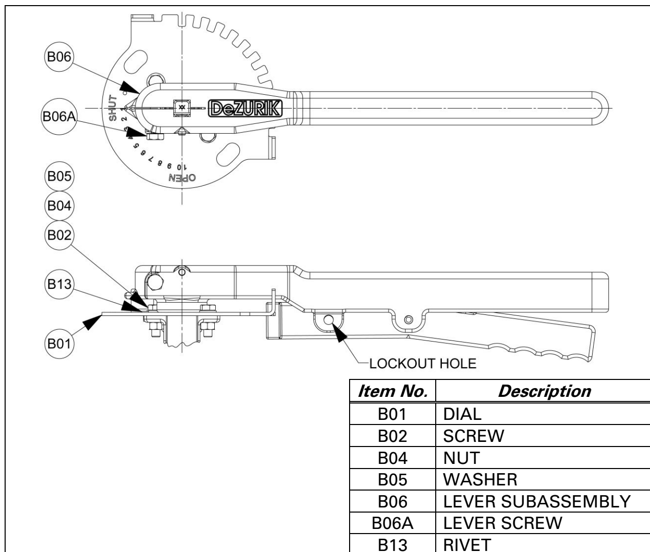
Figure 1 – Actuator Components
