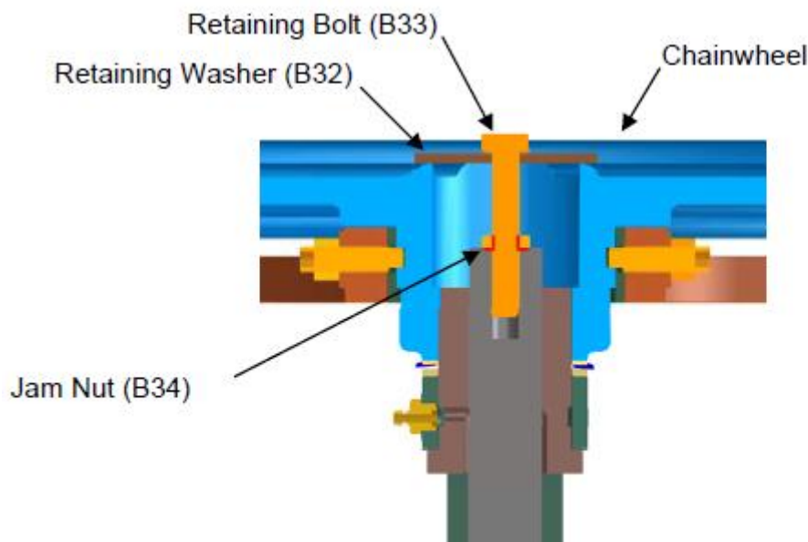
FIGURE 1—Detailed View of Chainwheel Retaining Components on 2-12" Valves
