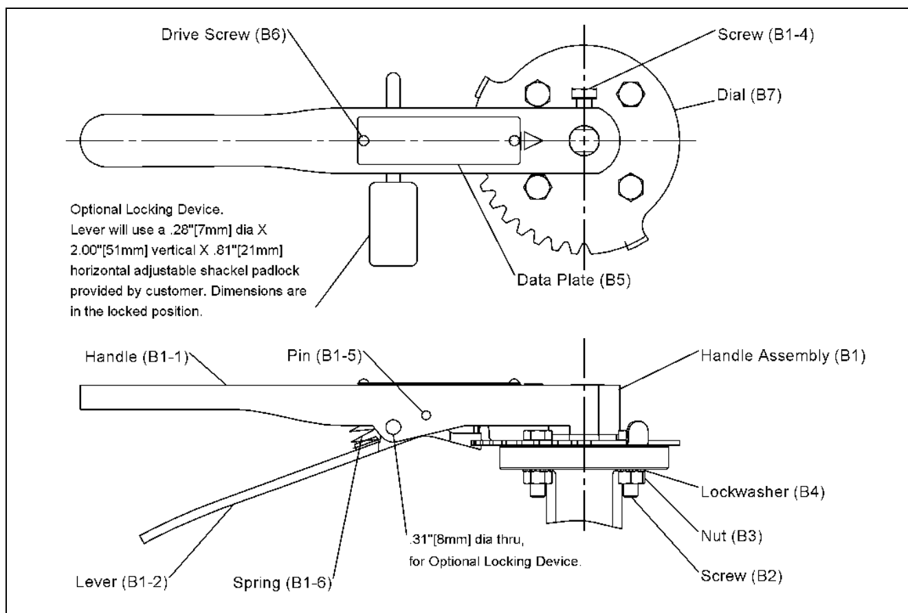
Figure 1— Parts Identification
