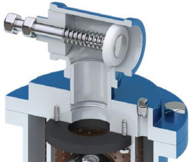
APCO Double Acting Throttling Device (DAT)
