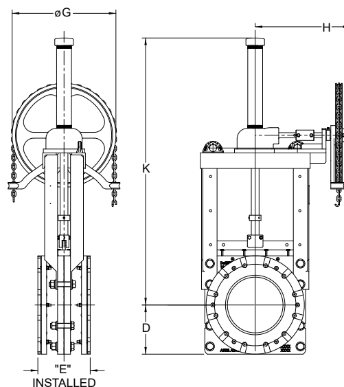
90 Degree Mounting
