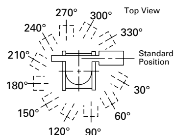
4-20" (100-500mm) Actuator Mounting Position
