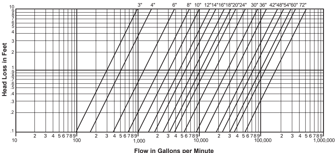
Actual Flow Test For Head Loss Characteristics
