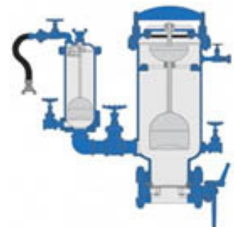
APCO ASV Dual Body Sewage Combination Air Valve Body Style 401C
