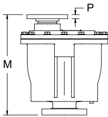
FL OPTION (FLANGE STYLE SAME AS INLET)
